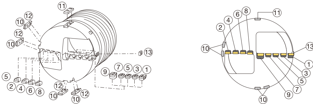
Part positions may vary depending on the drill size.
